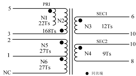
Figure 4:Transformer Electrical Diagram
