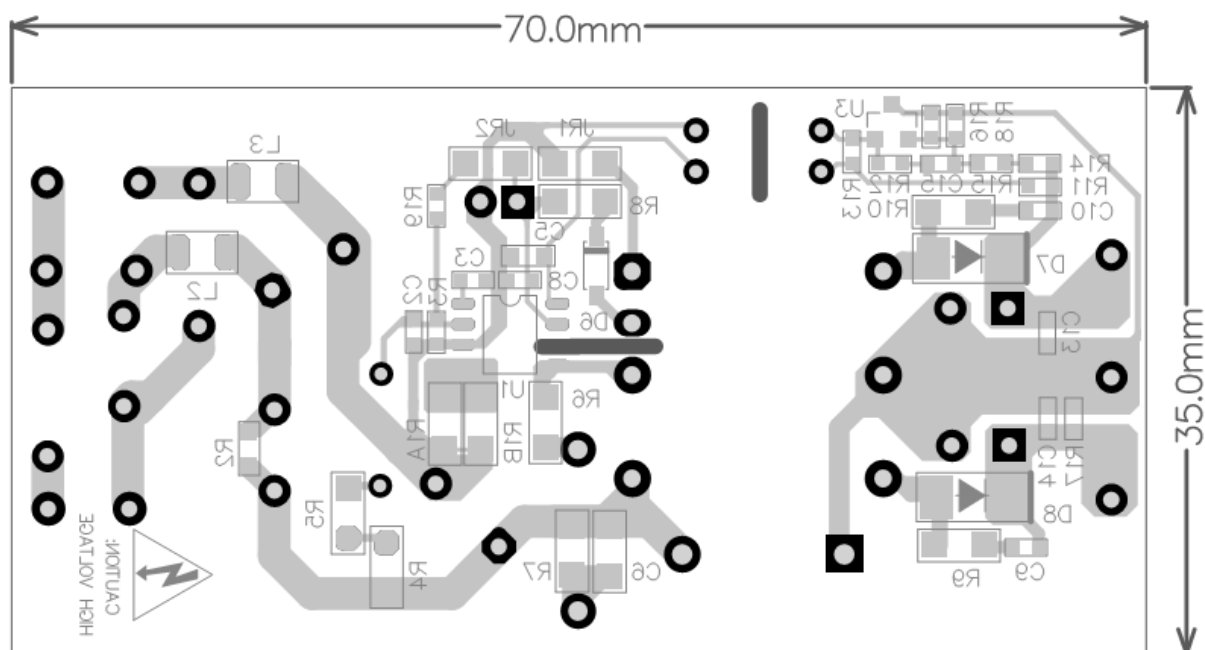
Figure 3: Bottom Layer
