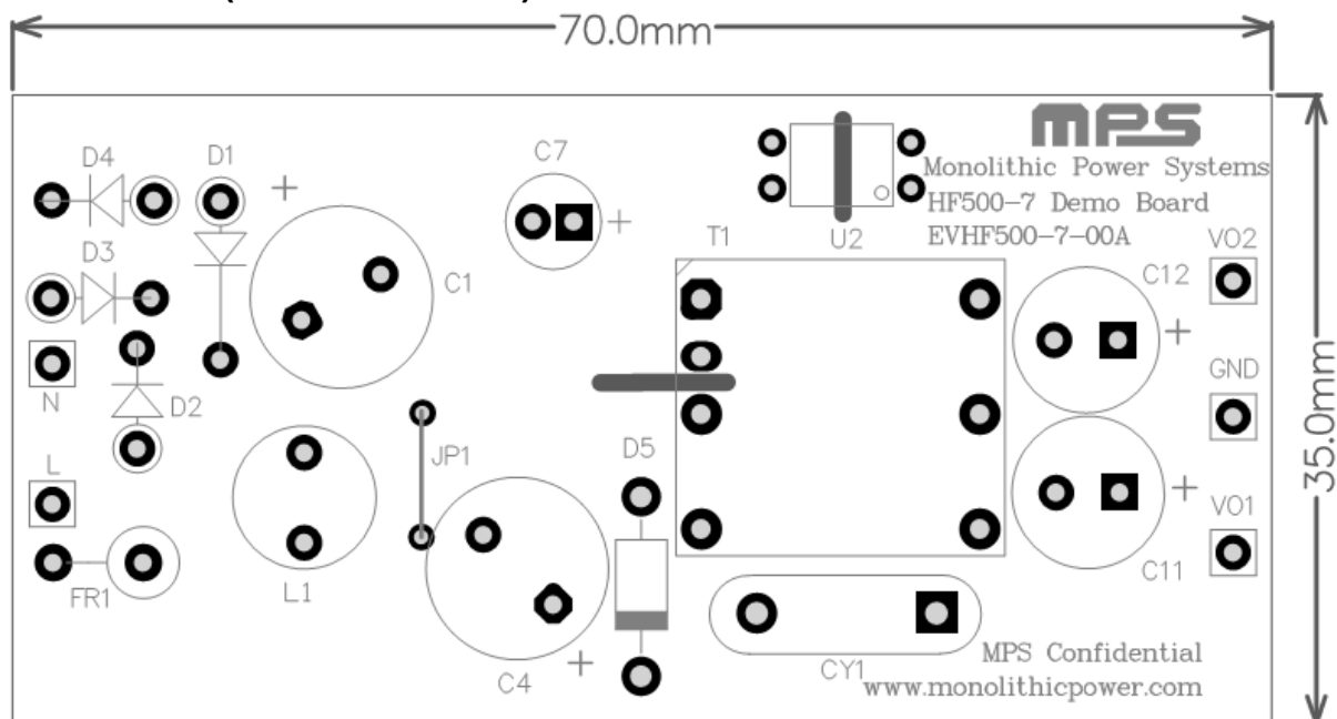
Figure 2: Top Layer
