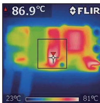
Thermal Performance V_{IN} = 85V_{AC}
