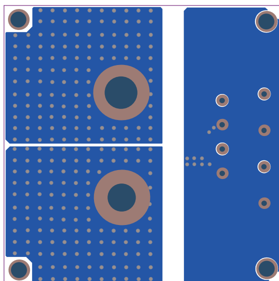
Figure 4: Bottom Layer
