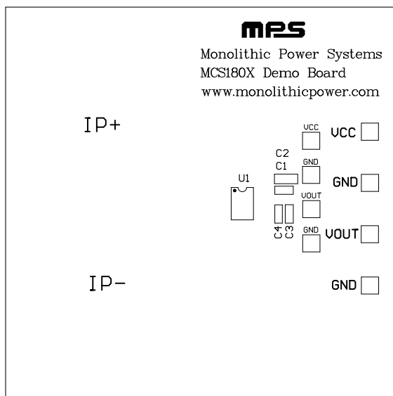
Figure 2: Top Silk
