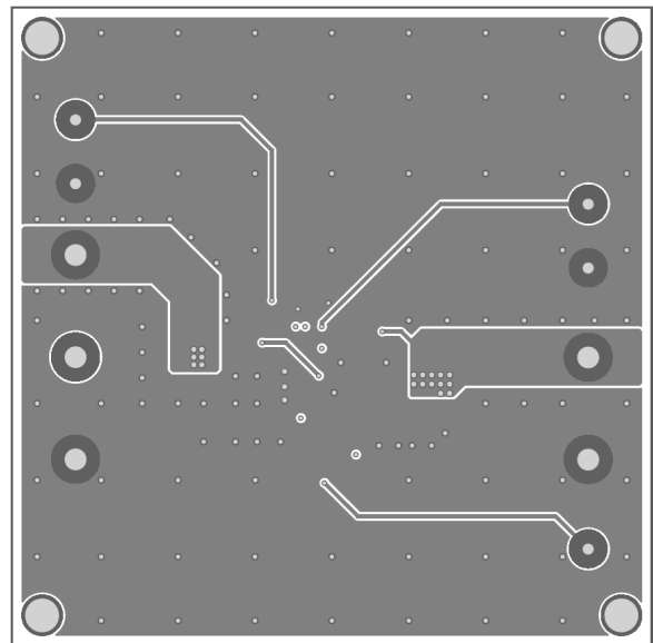
Figure 4: Inner2 Layer
