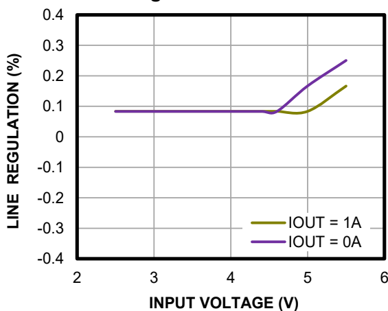
Line Regulation
