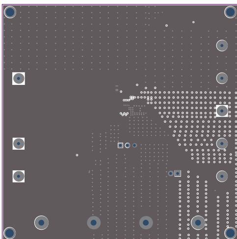
Figure 3: Inner 1 Layer
