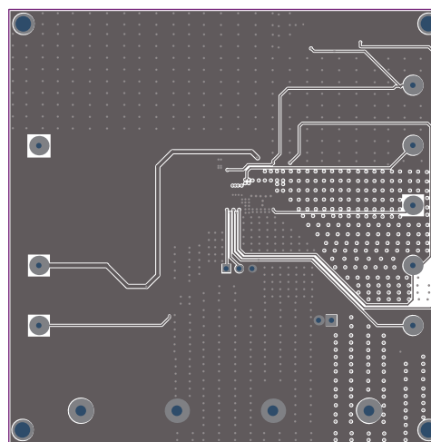
Figure 4: Inner 2 Layer
