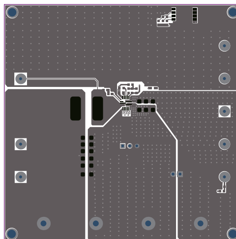
Figure 2: Top Layer
