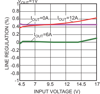
Line Regulation vs. Input Voltage
