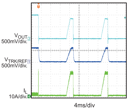
Over-Current
