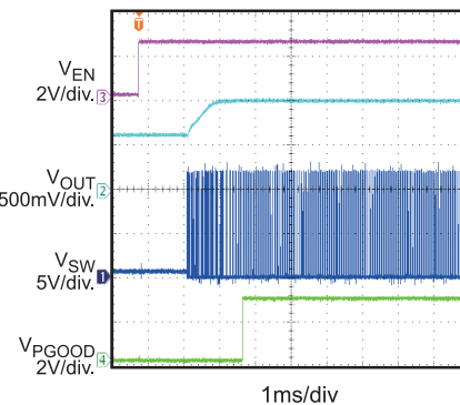
Pre-bias Start-Up
