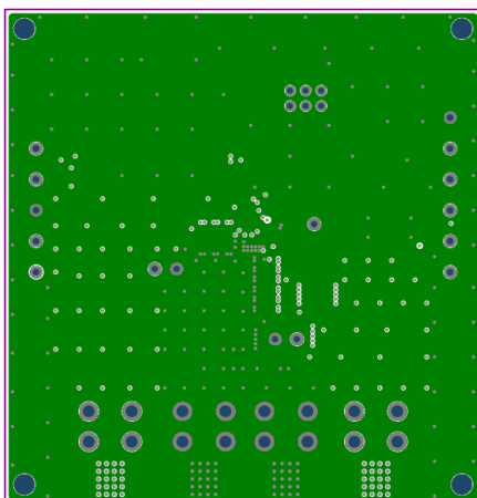
Figure 3—Inner Layer 1
