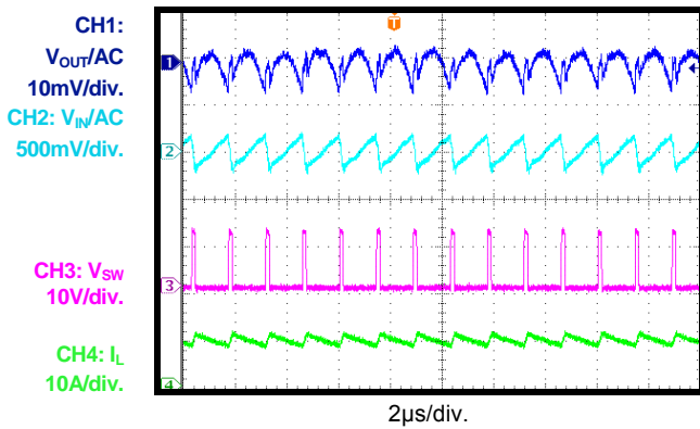
Input/Output Ripple I_{OUT}=10A
