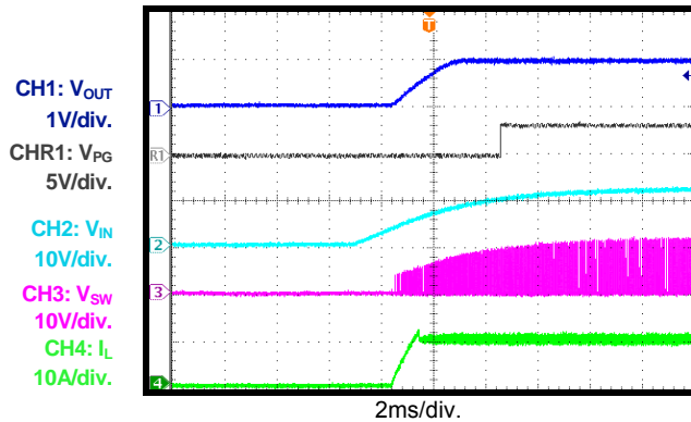
Start-Up through Input Voltage I_{OUT}=10A
