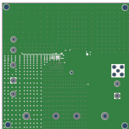
Figure 3—Inner Layer 1
