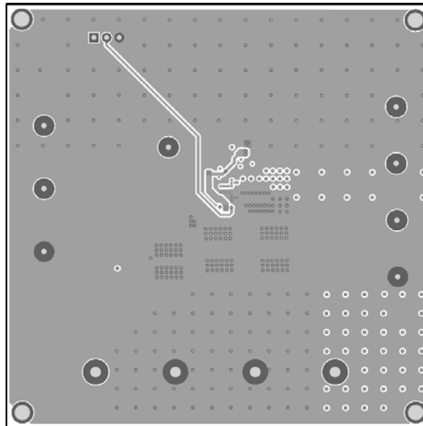
Figure 5: Bottom Layer
