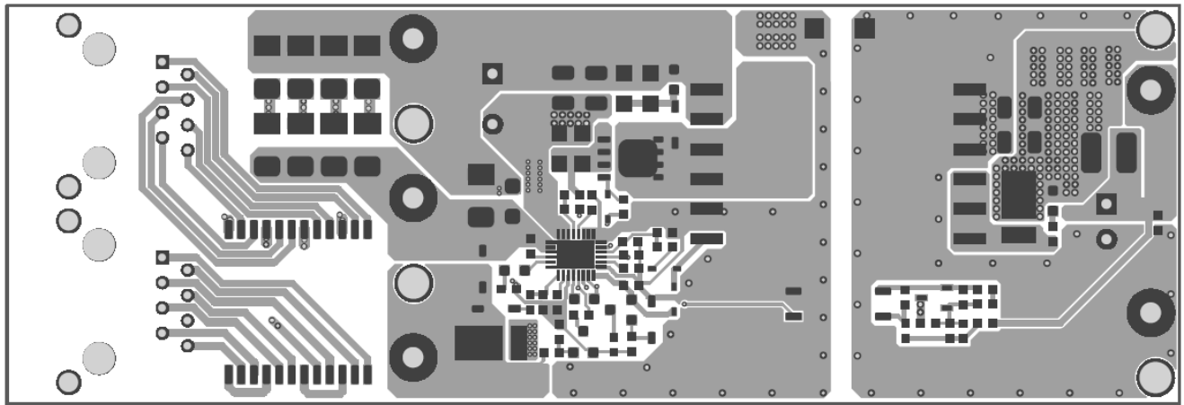
Figure 2: Top Layer
