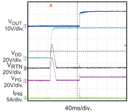
V DD Start-Up
