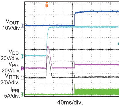
V DD Start-Up
