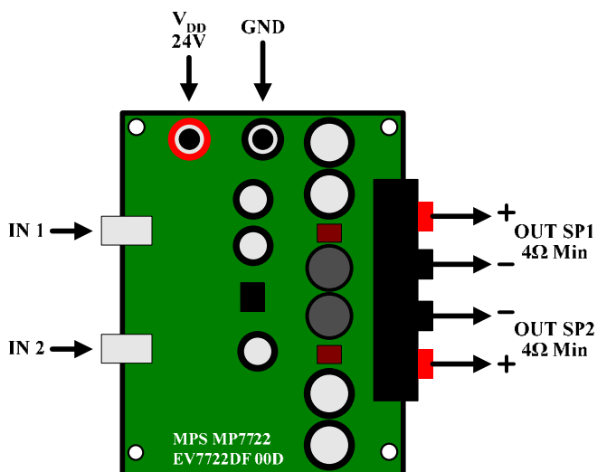
Figure 5—Connection Diagram
