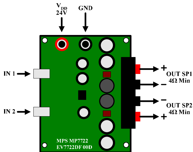
Figure 5—Connection Diagram
