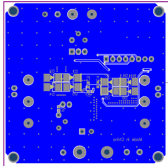
Figure 6: Bottom Silk
