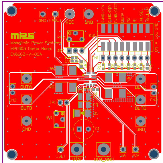
Figure 5: Top Silk
