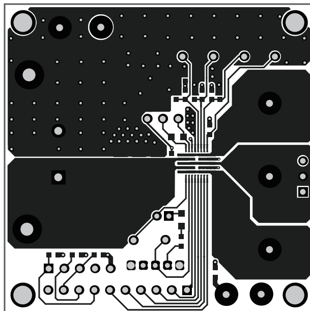
Figure 2: Top Layer
