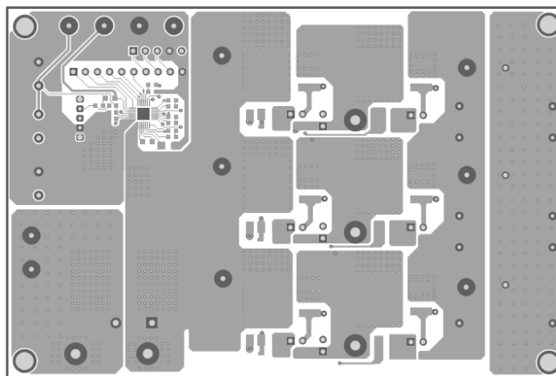
Figure 2: Top Layer
