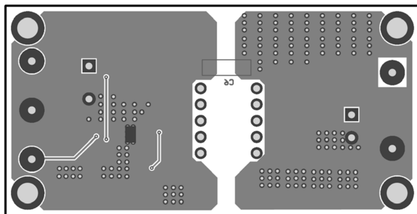
Figure 3: Bottom Layer
