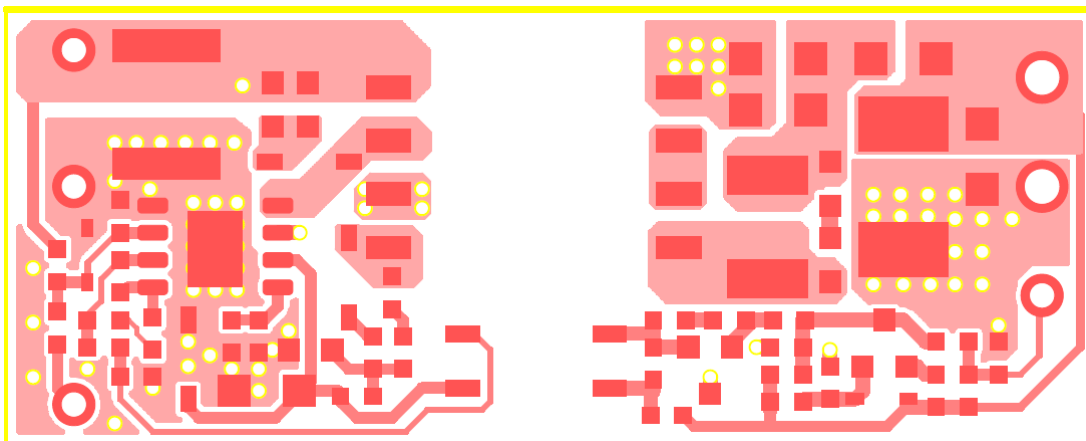
Figure 3: Top Layer
