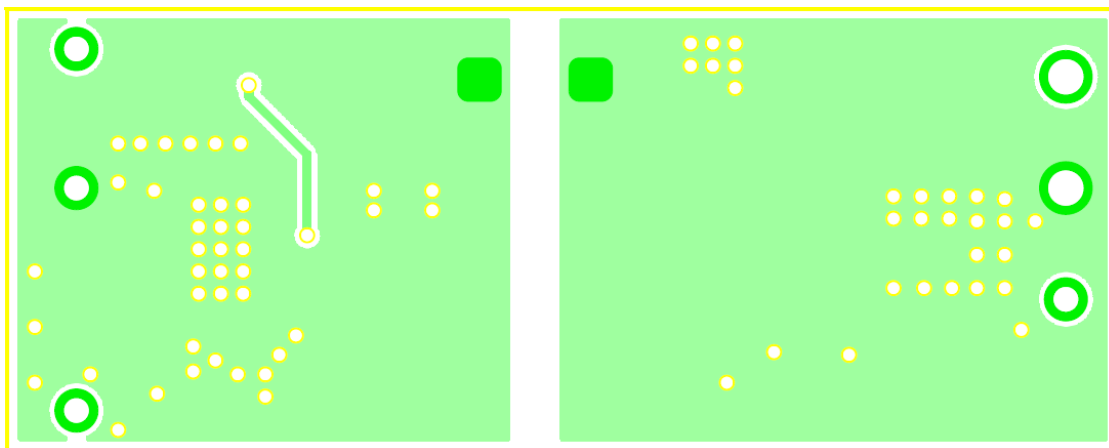
Figure 4: Bottom Layer
