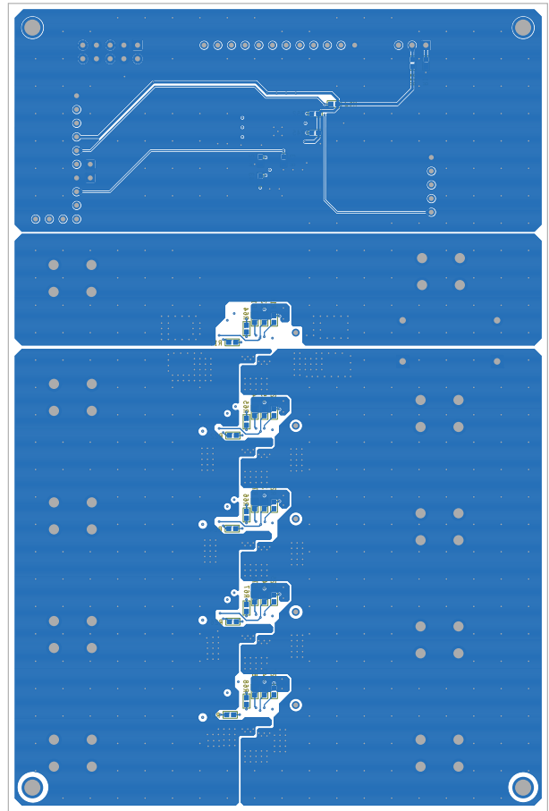
Figure 14: Bottom Layer
