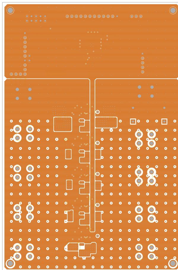
Figure 12: Mid-Layer 1
