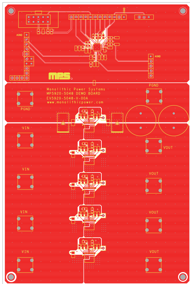
Figure 11: Top Layer
