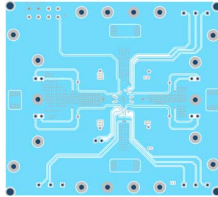
Figure 4: Middle Layer 2
