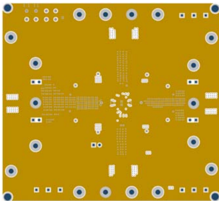
Figure 3: Middle Layer 1
