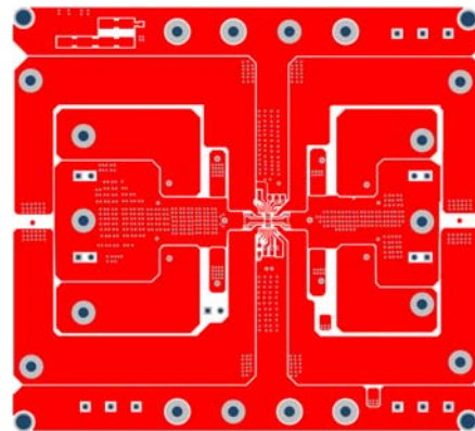
Figure 2: Top Layer
