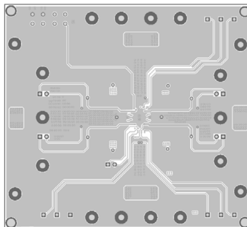
Figure 4—Inner Layer2
