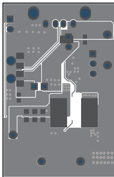
Figure 2: Top Layer
