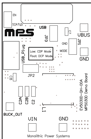
Figure 1: Top Silk Layer
