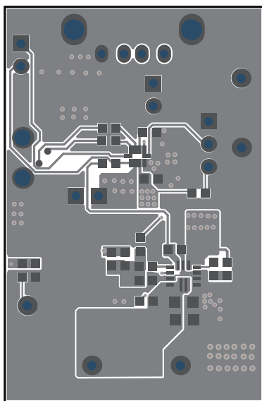
Figure 3: Bottom Layer
