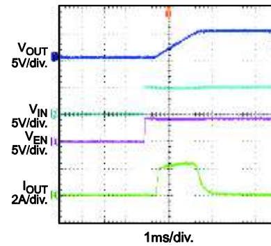
Start-Up through Input Voltage I_{LOAD}=0A , C_{OUT}=1000\mu F
