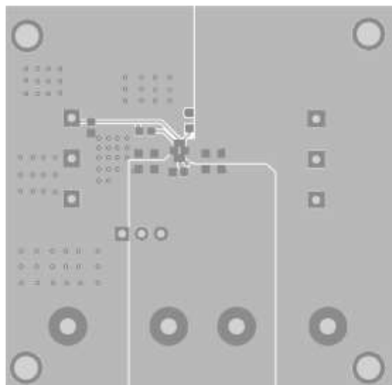
Figure 2: Top Layer
