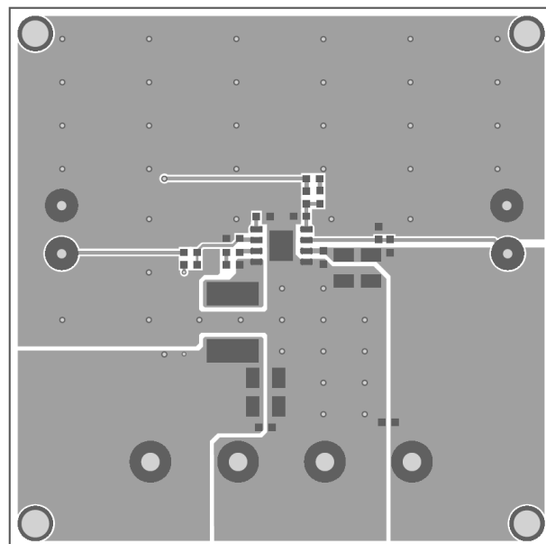
Figure 2 – Top Layer
