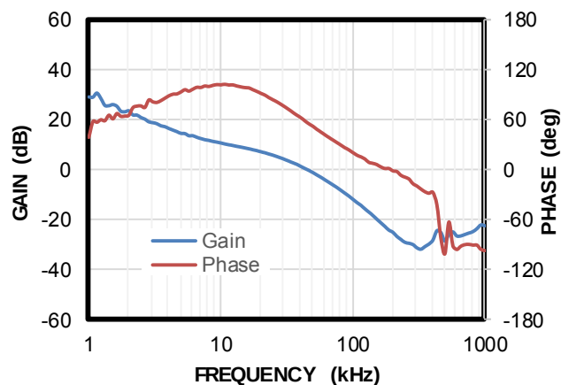
Bode Plot
