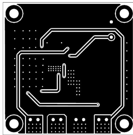
Figure 4—Inner 2 Layer
