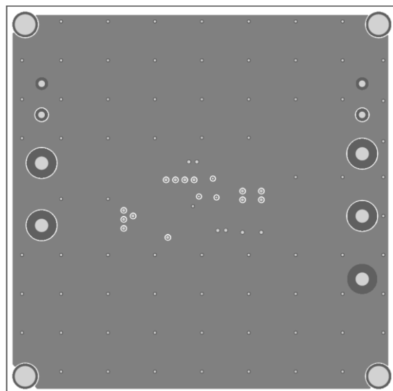
Figure 2—Inner1 Layer
