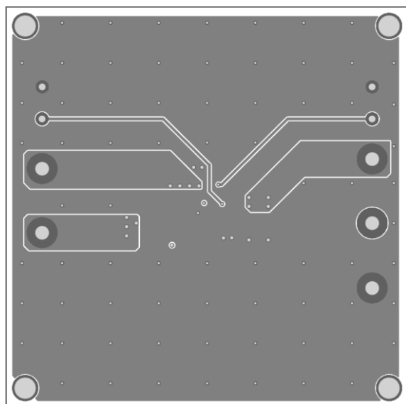
Figure 3—Inner2 Layer
