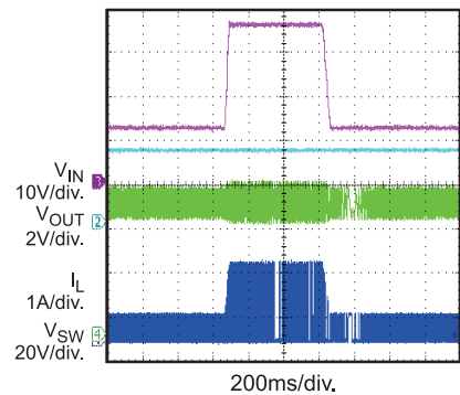
Load Dump
