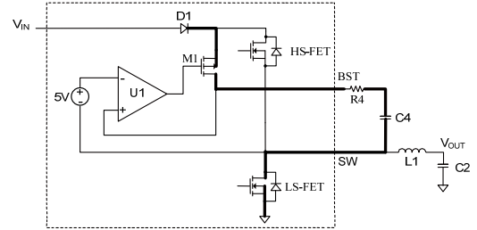
3a: BST Charging Path when LS-FET is On
