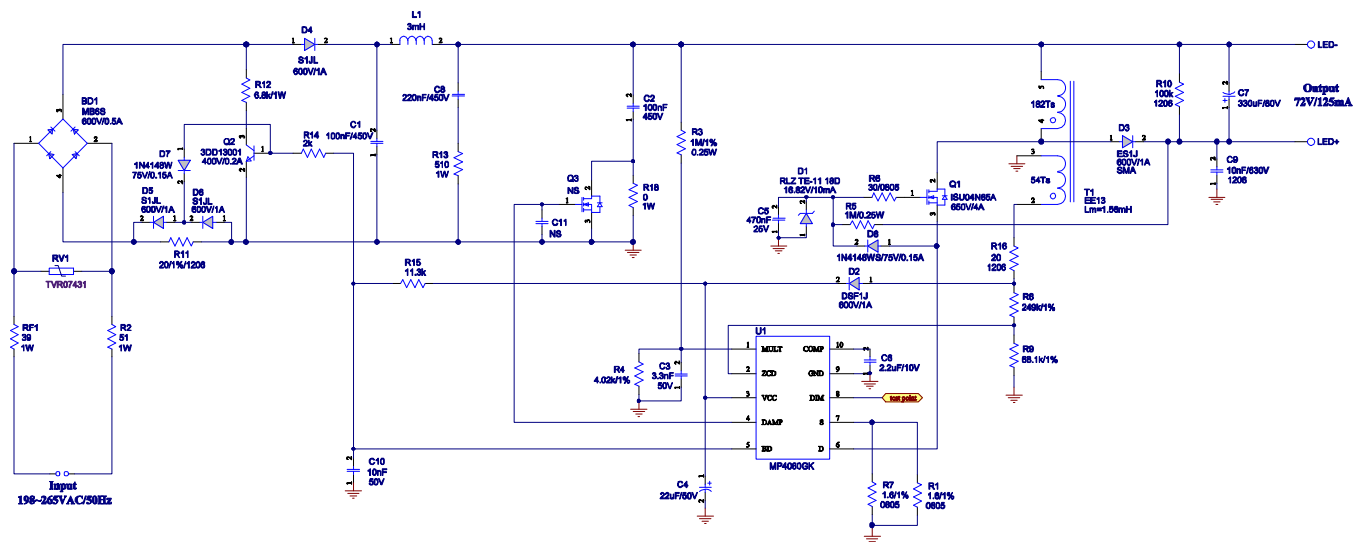
Figure 1—Schematic
