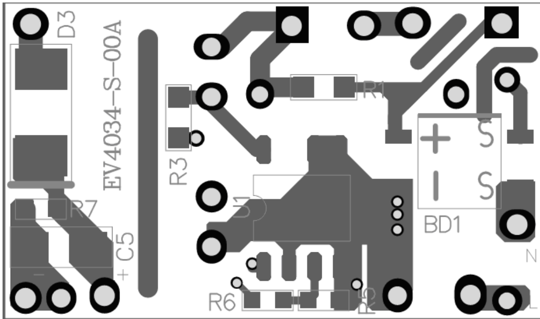
Figure 3: Bottom Layer
