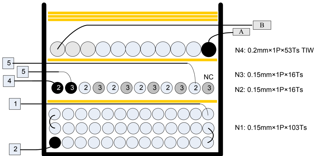
Figure 5: Winding Diagram
