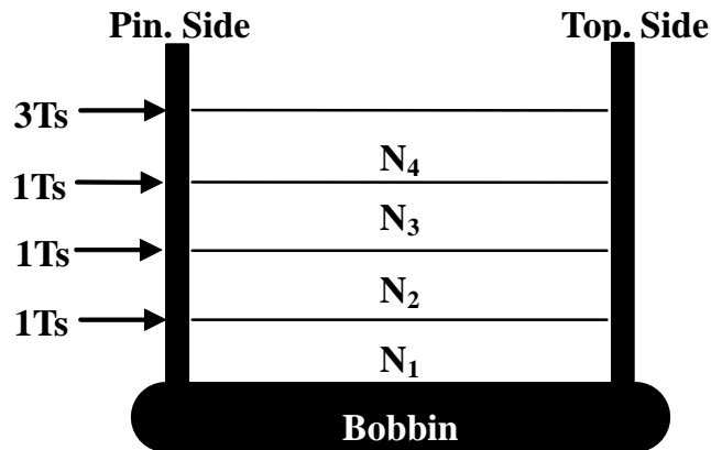
Figure 5—Winding Diagram
