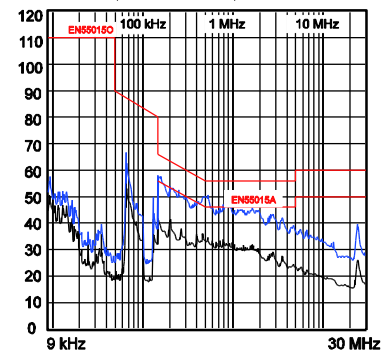
Conduction EMI
