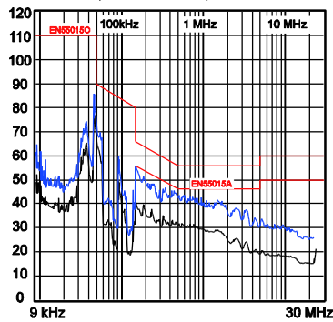
Conduction EMI
