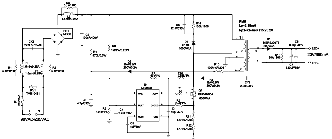
Figure 1 - Schematic
