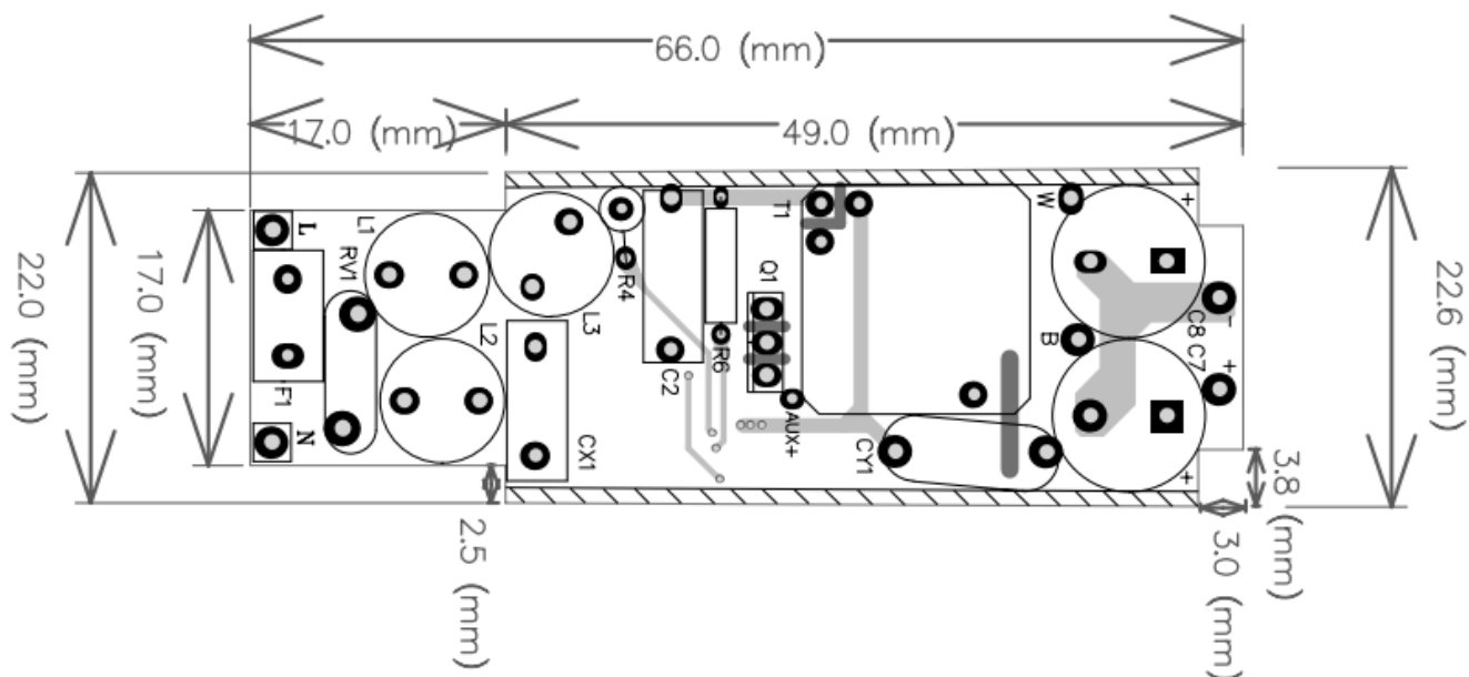
Figure 2 - Top Layer
