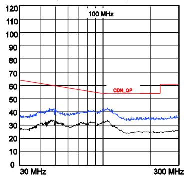
CDN Test
