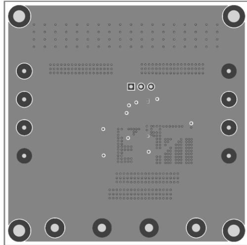
Figure 4—Inner Layer 2
