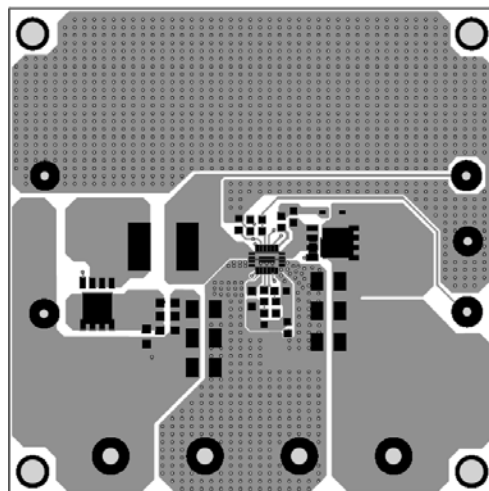
Figure 2: Top Layer
