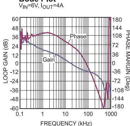
Bode Plot
