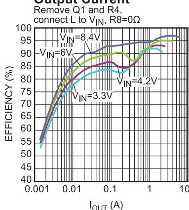
Efficiency vs. Output Current
