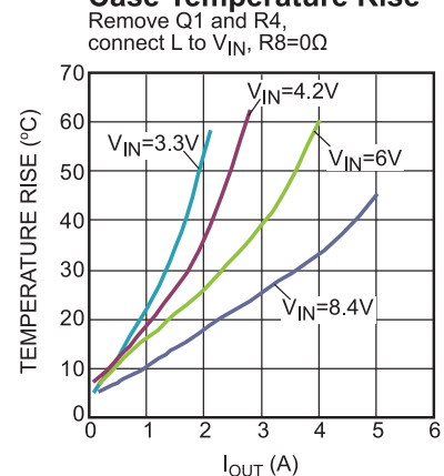
Case Temperature Rise
