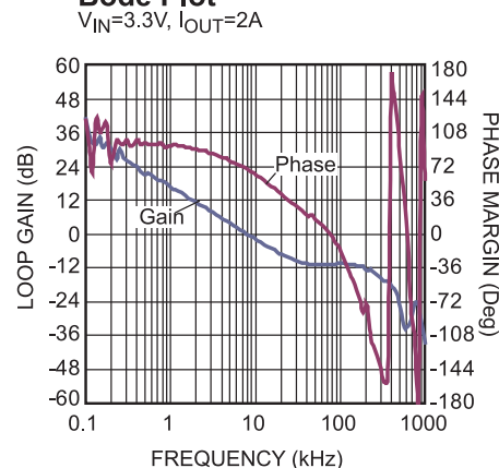
Bode Plot
