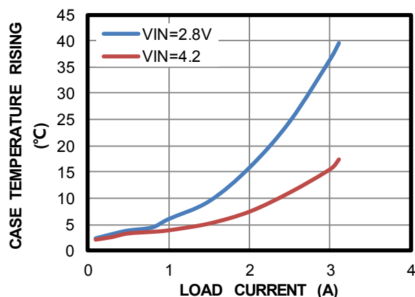
Case Temperature Rising vs. Load Current
