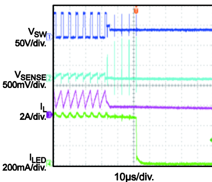
Short-Inductor Protection
