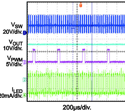
Dimming in Mix Mode
