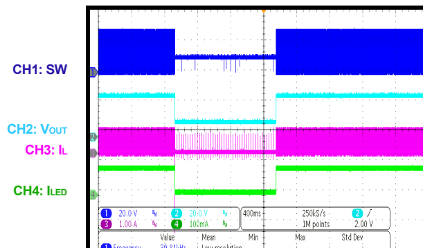
Short Diode When Work Normal Then Recover
