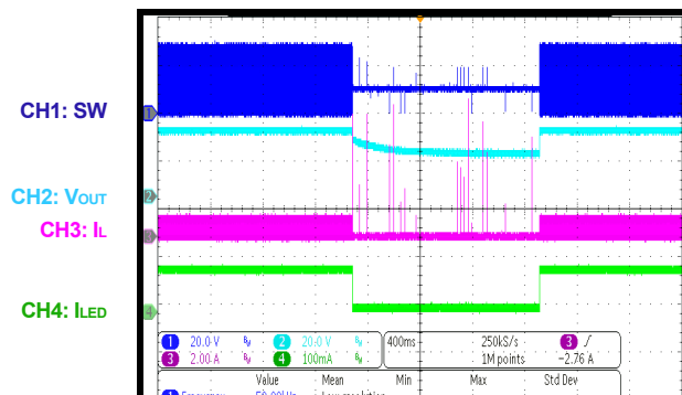
Short Inductor When Work Normal Then Recover
