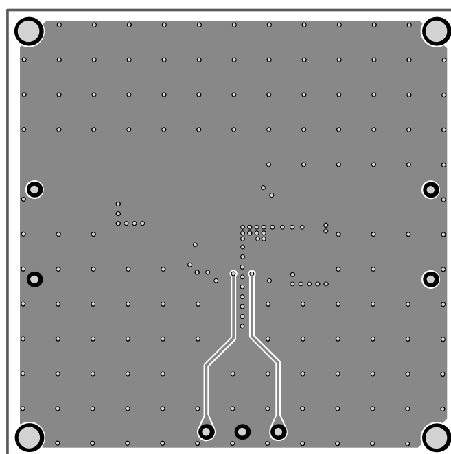
Figure 2: Bottom Layer
