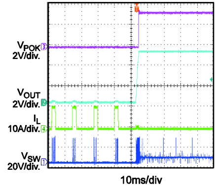
SCP Recovery short circuit to I_{OUT}=0
