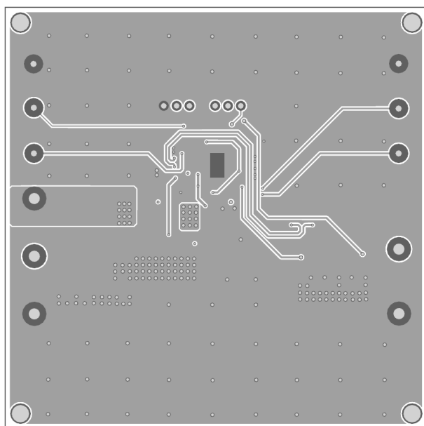
Figure 4—Inner Layer 2
