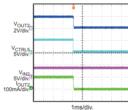
CTRL Off I_{OUT2} = 0.1A
