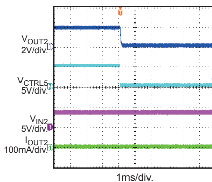
CTRL Off I_{OUT2} = 0A
