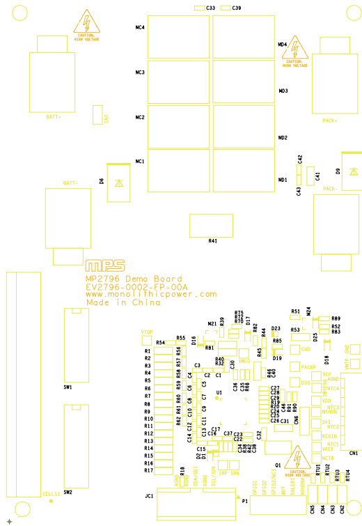
Figure 56: Top Silk
