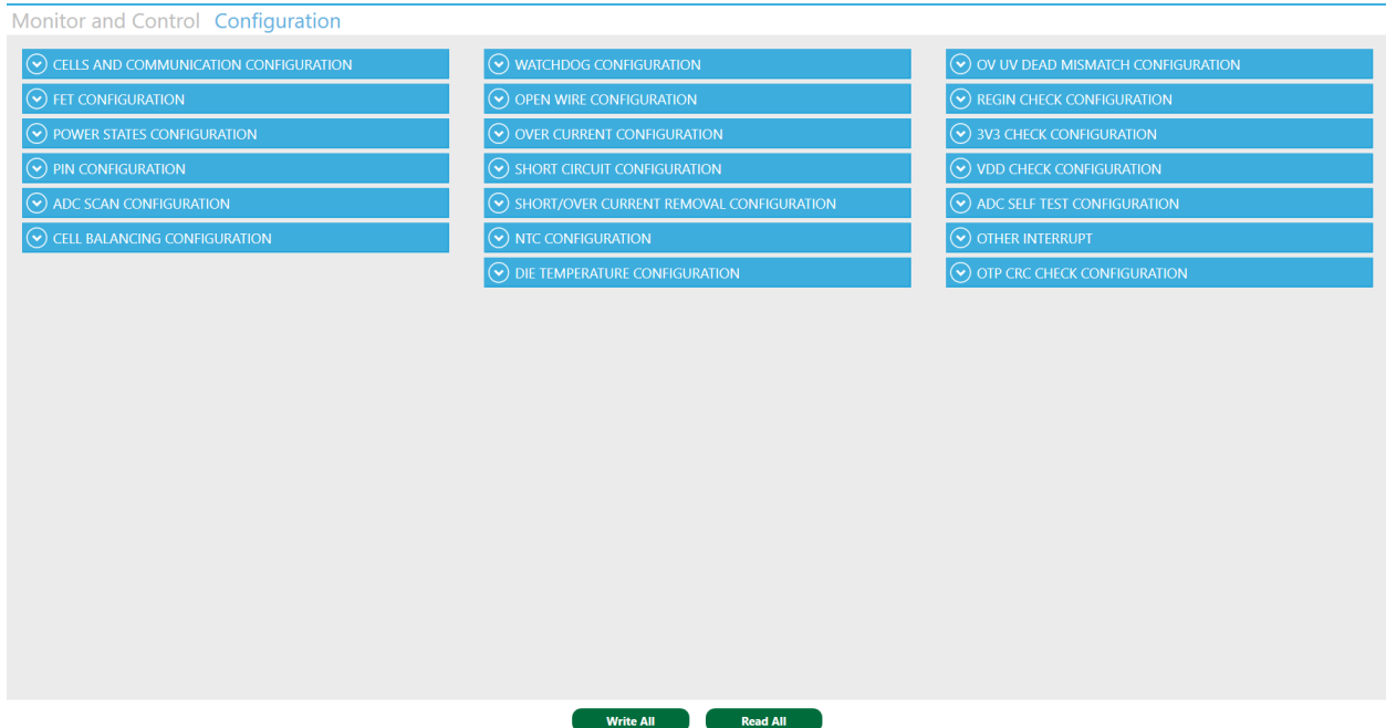
Figure 9: Configuration View
