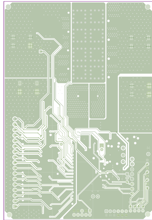
Figure 59: Mid-Layer 2
