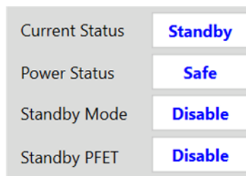
Figure 34: Status Monitor
