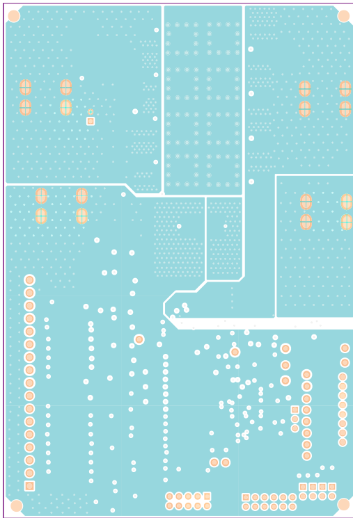
Figure 58: Mid-Layer 1
