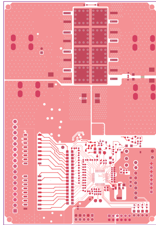
Figure 57: Top Layer
