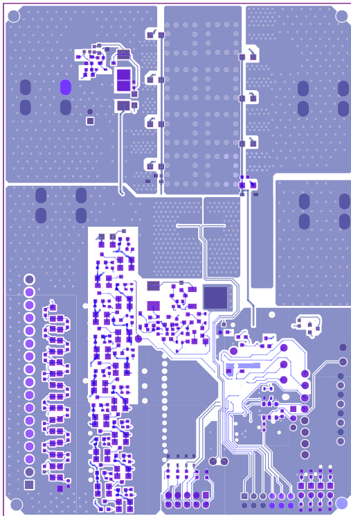
Figure 54: Bottom Layer
