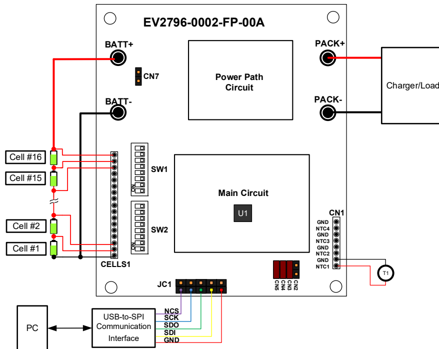
Figure 7: Test Set-Up for the MP2796DFP-0002 with a Battery Pack
