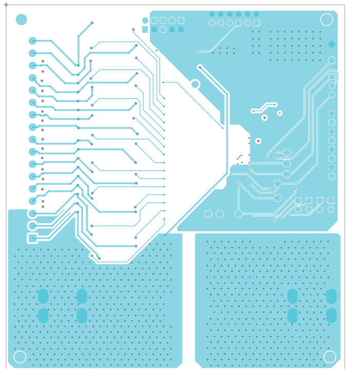
Figure 53: Mid-Layer 2
