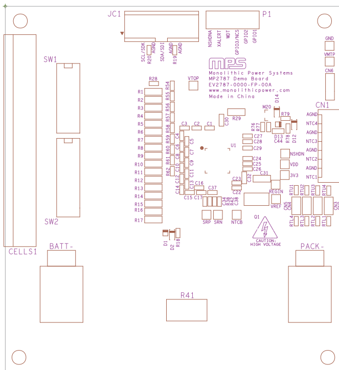
Figure 44: Top Silk
