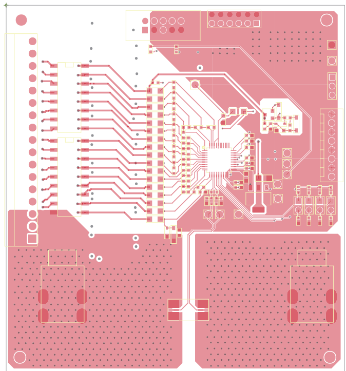
Figure 51: Top Layer
