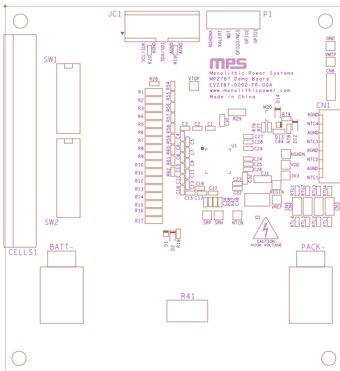
Figure 50: Top Silk
