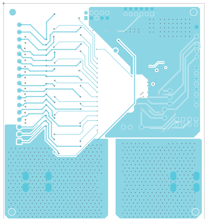
Figure 47: Mid-Layer 2
