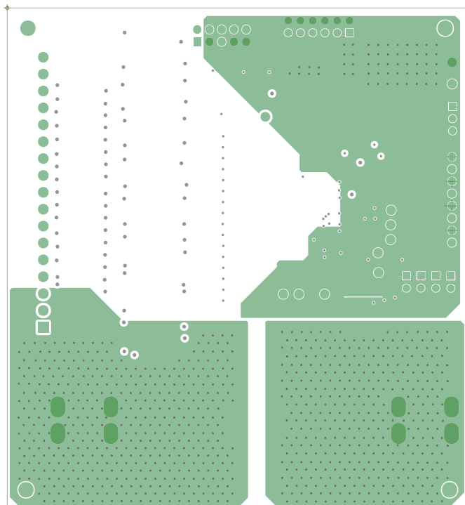
Figure 52: Mid-Layer 1
