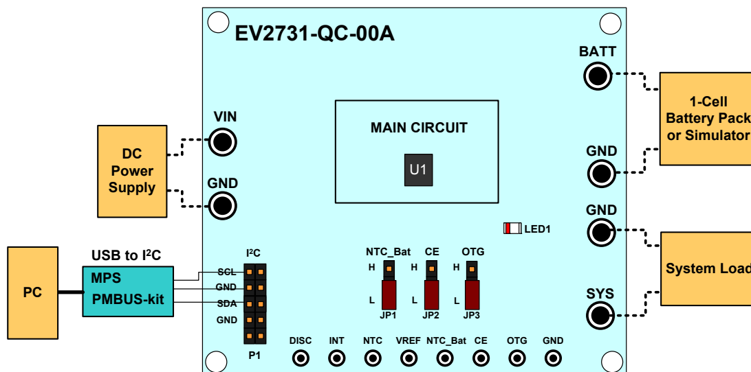
Figure 2: Test Set-Up for the MP2731
