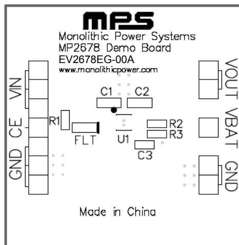
Figure 2: Top Silk
