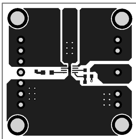
Figure 3: Top Layer
