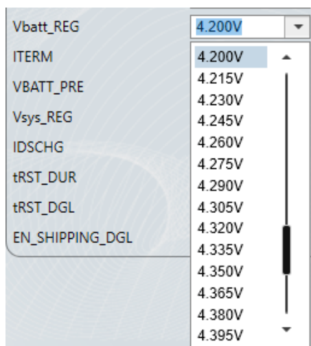
Figure 11: Battery Regulation Voltage Setting
