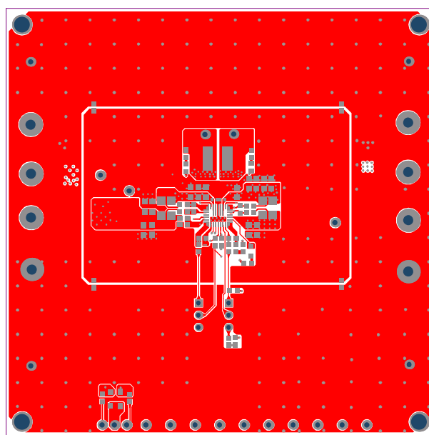
Figure 26: Top Layer
