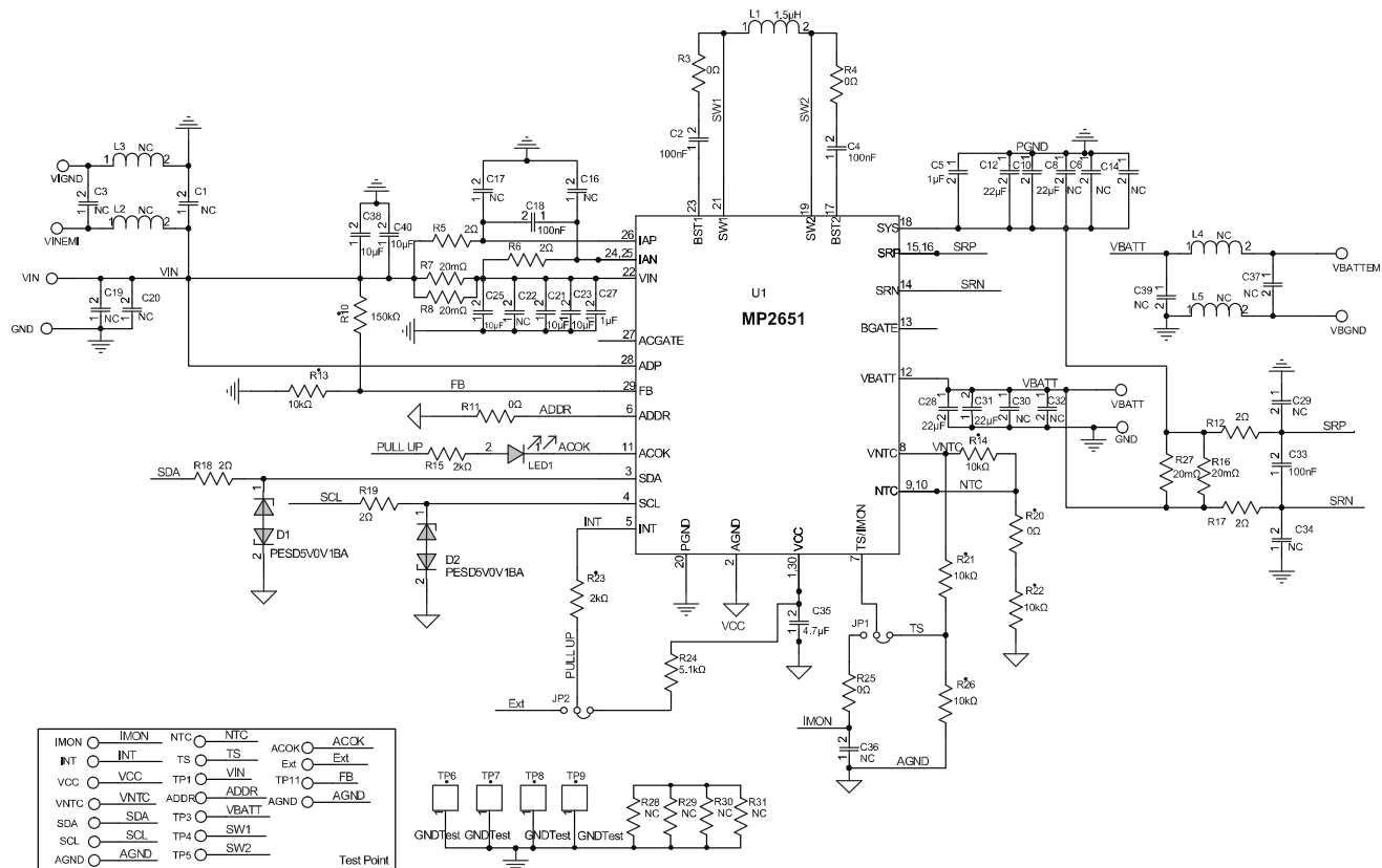
Figure 24: Evaluation Board Schematic
