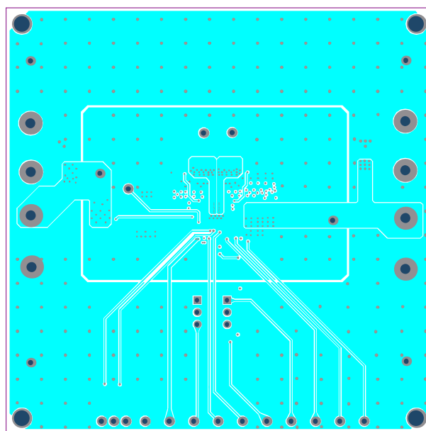
Figure 28: Mid-Layer 2
