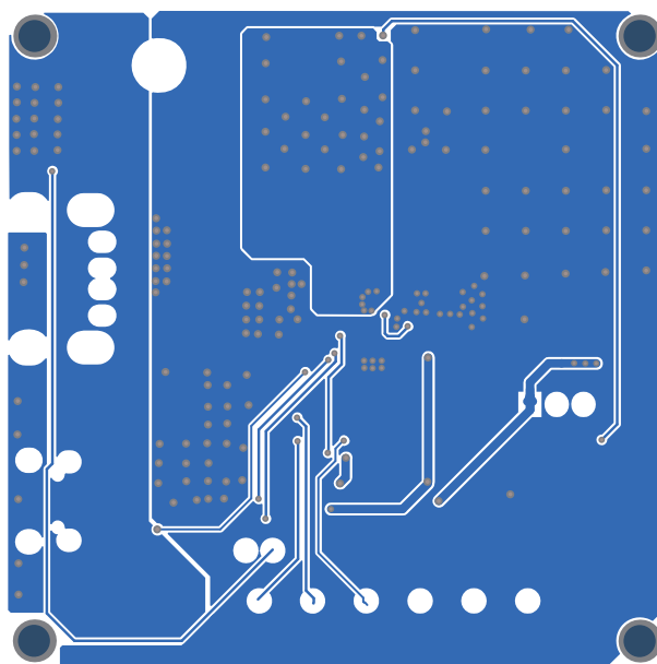
Figure 2: Bottom Layer
