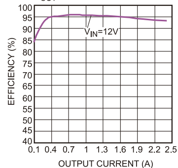
Efficiency vs. Output Current V OUT =5V
